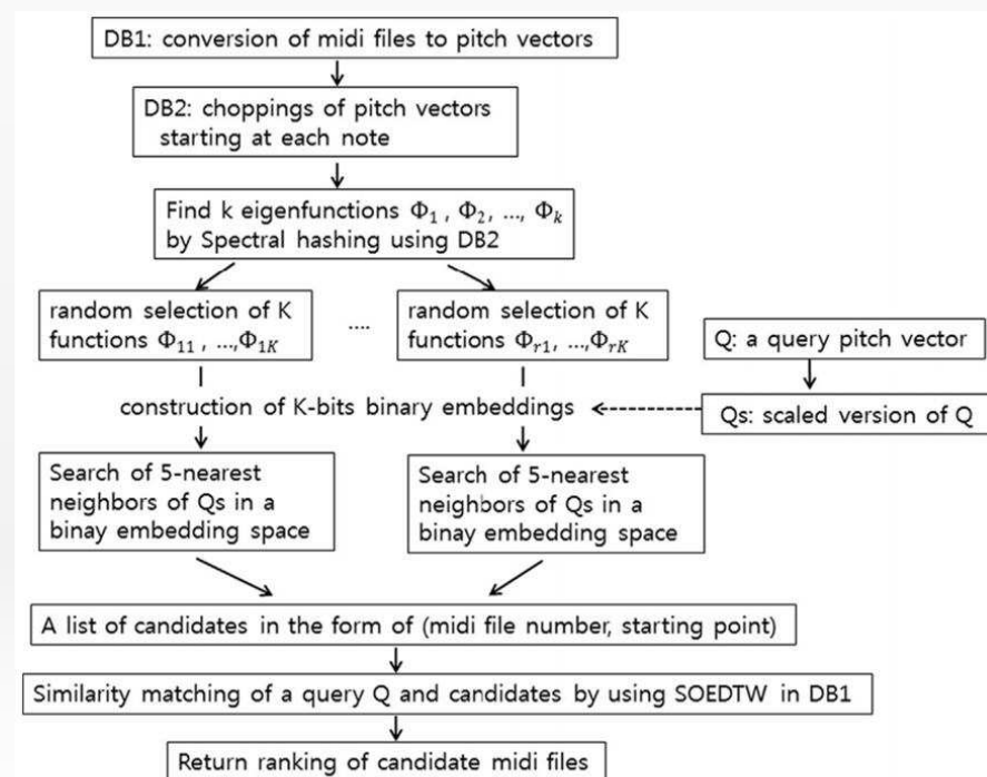
Fig. 1. A flowchart of the proposed QBH method.
