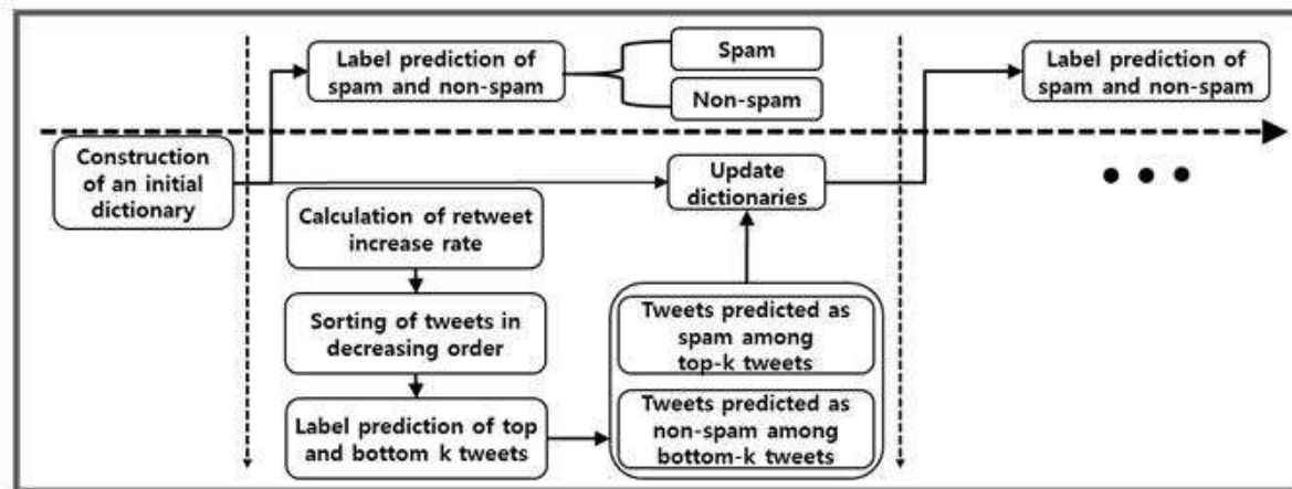
Figure 3. A flowchart of the proposed method when an initial training set is small
